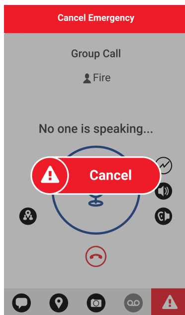
Figure 56: Cancel Emergency
