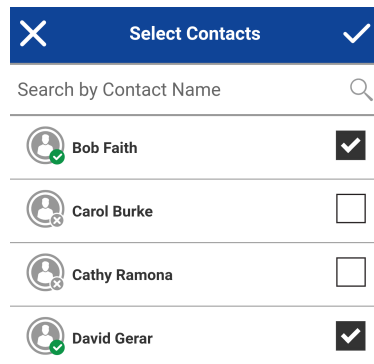
Figure 197: Select Contacts
