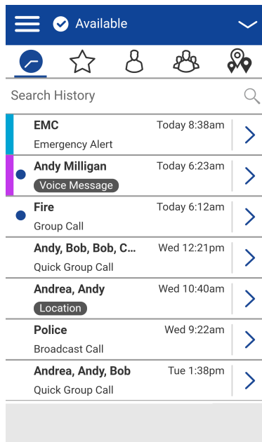
Figure 189: History
