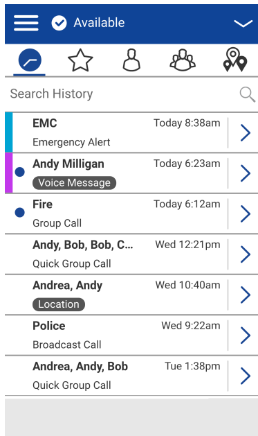
Figure 36: History
