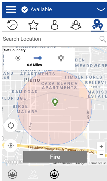
Figure 157: Boundary ON
