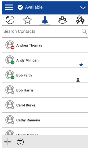
Figure 16: Contacts
