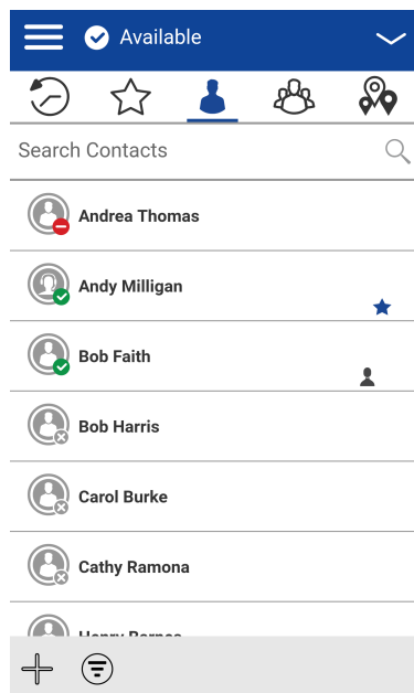
Figure 25: Contacts
