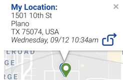
Figure 139: My Location
