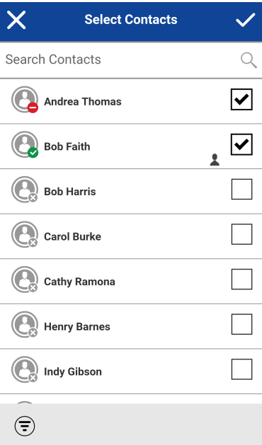
Figure 27: Select Contacts
