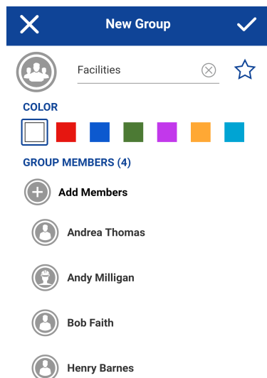
Figure 114: New Group
