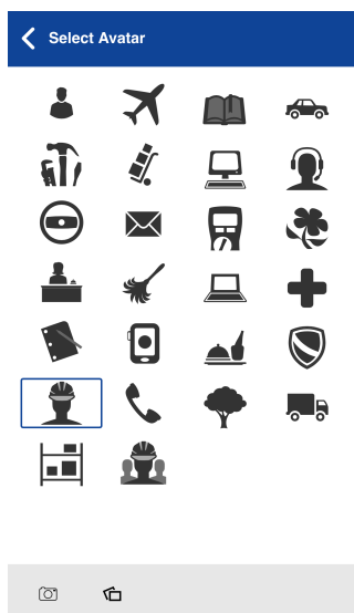
Figure 101: Select Avatar
