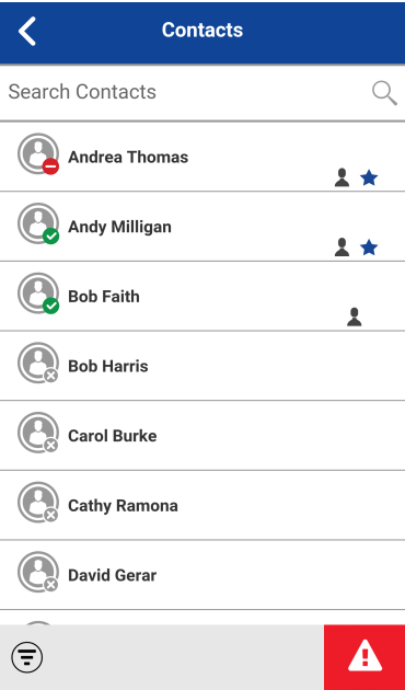
Figure 58: Contacts
