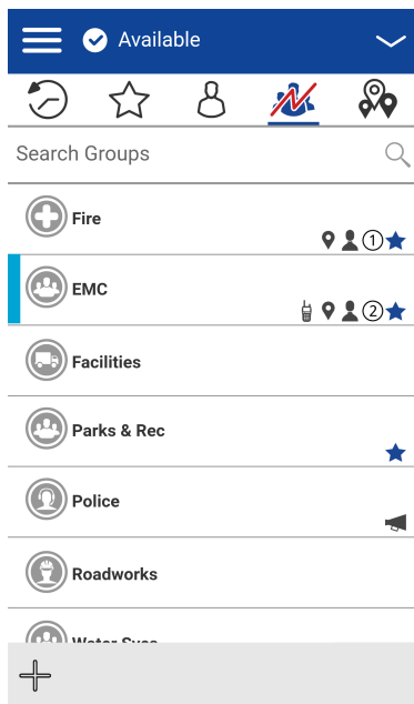
Figure 129: Talkgroup Scanning
