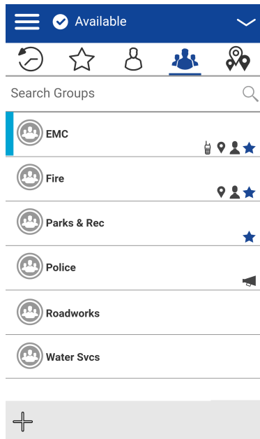
Figure 12: Groups
