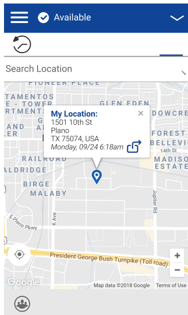
Figure 167: Map
