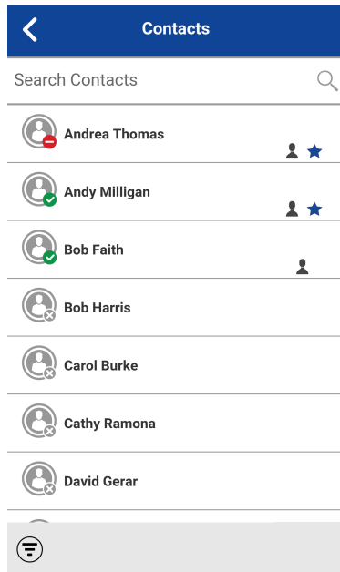
Figure 89: Contacts
