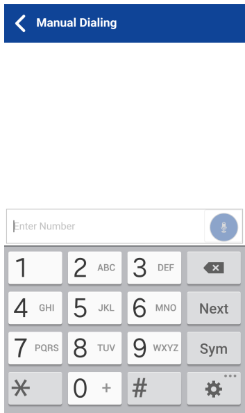
Figure 40: Manual Dial
