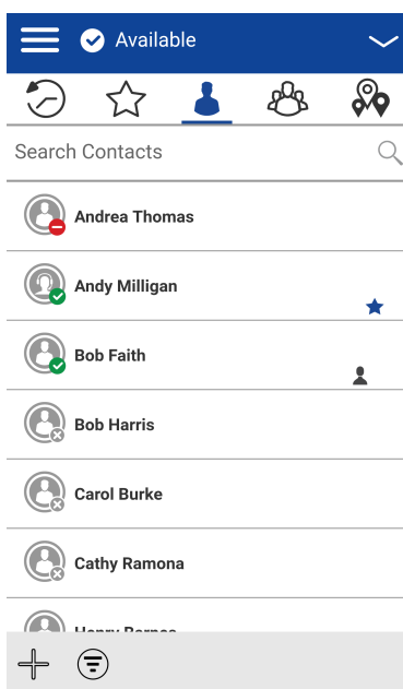
Figure 11: Contacts
