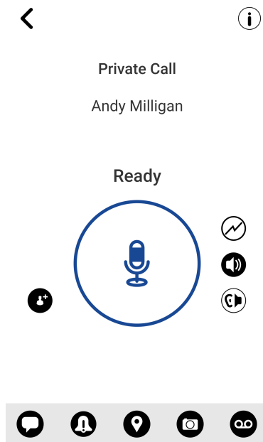
Figure 48: Call screen
