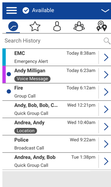
Figure 9: History
