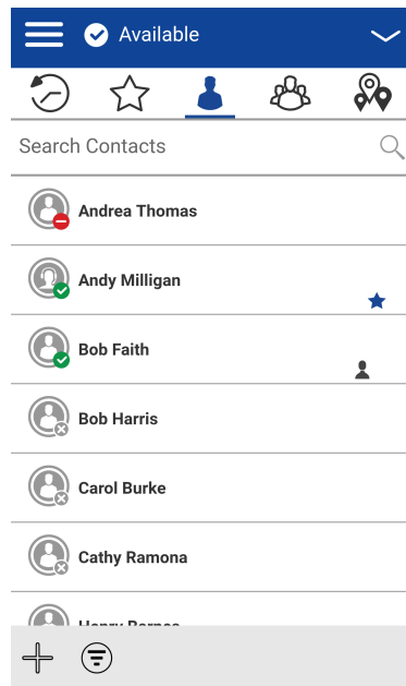
Figure 73: Contacts
