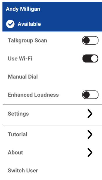
Figure 15: Menu Options
