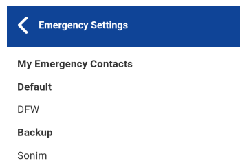
Figure 223: Emergency Setting
