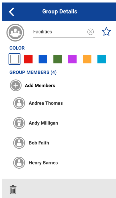
Figure 115: Group Details
