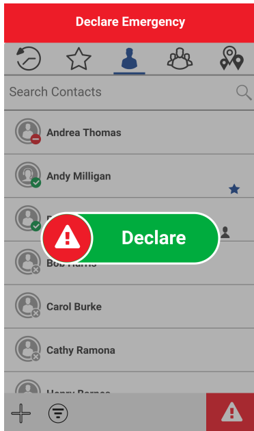
Figure 50: Declare Emergency
