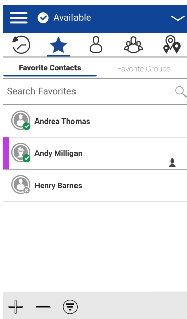
Figure 10: Favorites
