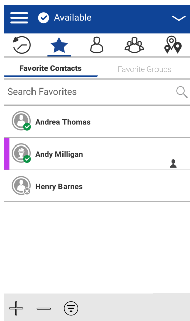
Figure 84: Favorite Contacts
