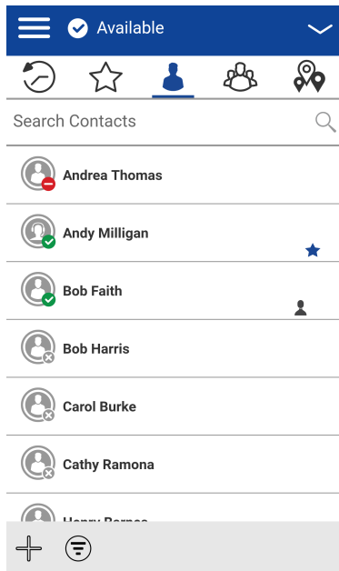
Figure 192: Contacts
