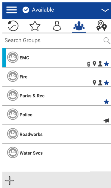
Figure 71: Supervisor Talkgroup
