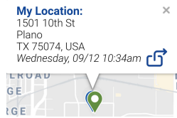
Figure 142: My Location
