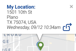
Figure 145: My Location
