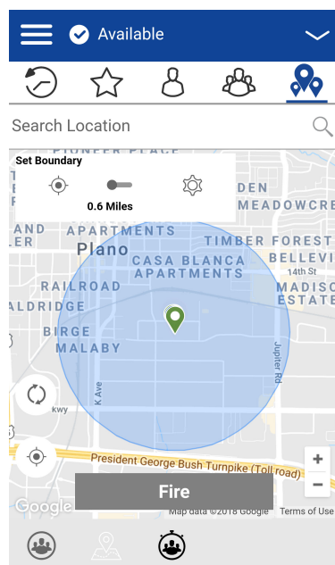
Figure 155: Boundary Preview
