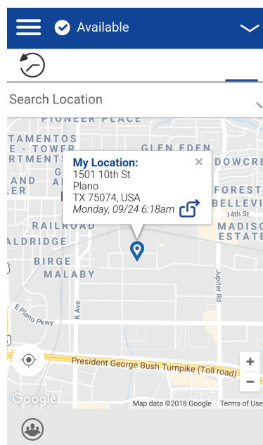
Figure 13: Map
