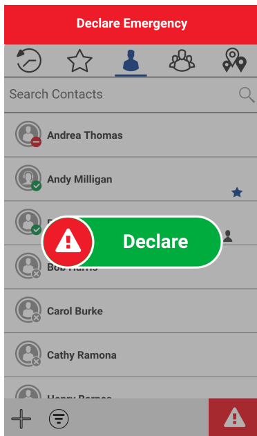
Figure 61: Declare Emergency
