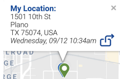
Figure 153: My Location
