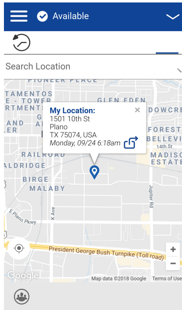
Figure 138: Map
