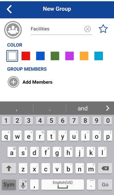
Figure 112: New Group
