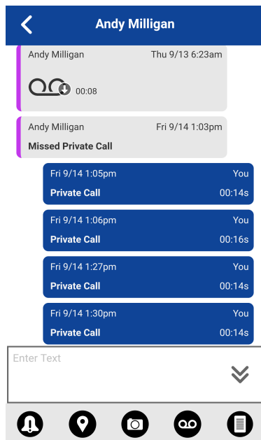
Figure 190: History Details
