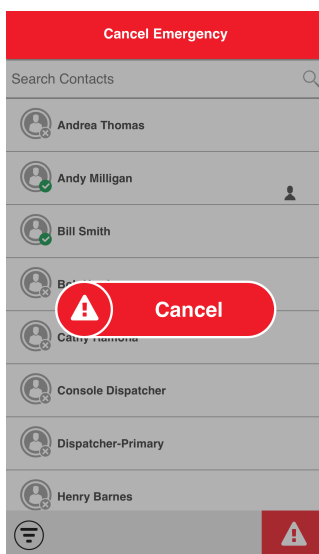
Figure 65: Cancel Emergency
