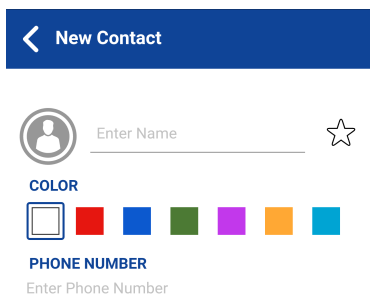
Figure 98: New Contact
