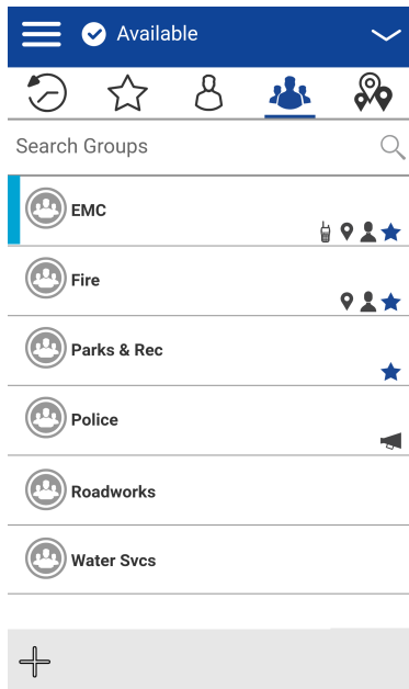
Figure 21: Talkgroups
