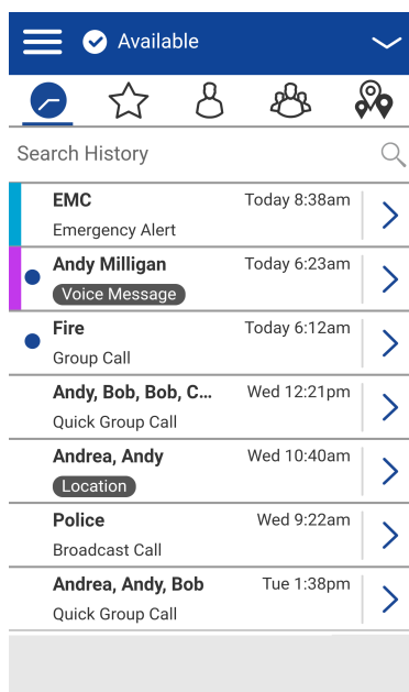
Figure 83: History
