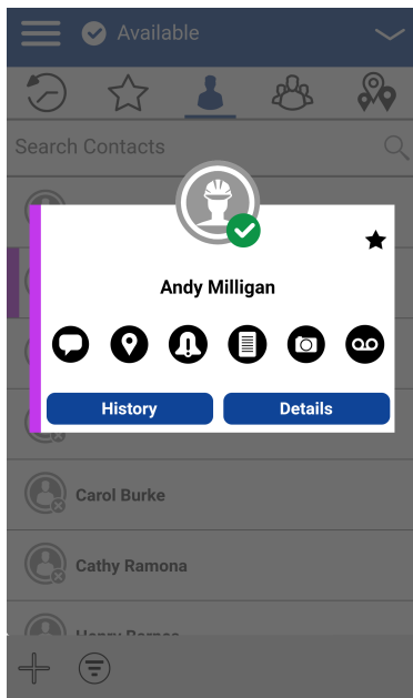
Figure 95: Context Menu
