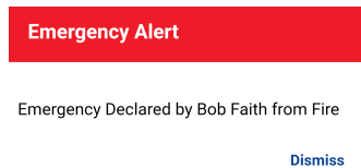
Figure 54: Emergency Alert
