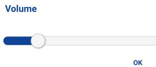
Figure 47: Volume Control
