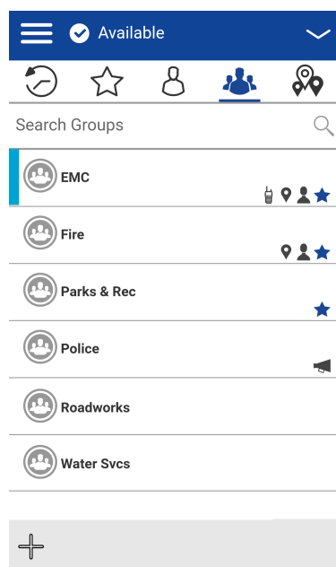
Figure 30: Talkgroups
