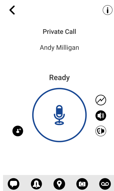
Figure 14: Call screen
