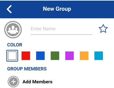
Figure 111: New Group
