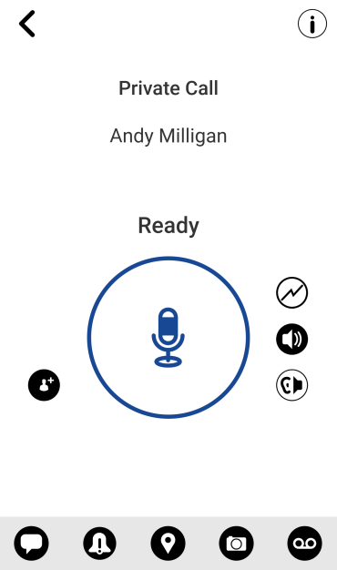
Figure 26: Call screen
