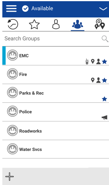
Figure 107: Talkgroups
