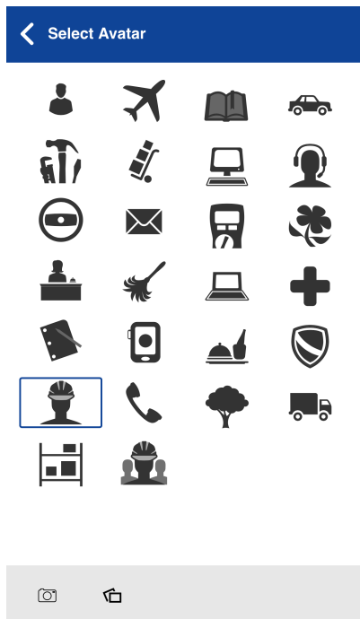
Figure 122: Select Avatar
