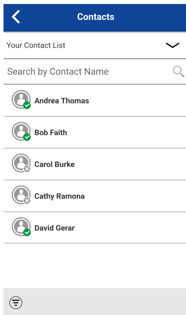
Figure 195: Contacts
