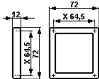
Glass for measuring instrument AM 72
