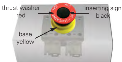
Mushroom-head pushbutton actuator "EMERGENCY STOP" GHG 410 1437R....
